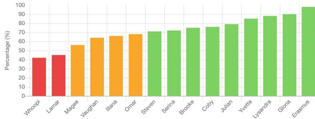
Student Scores
